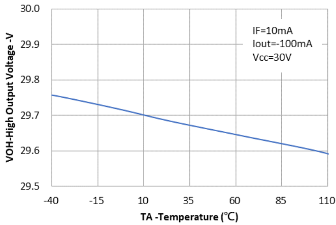
Fig.1 High output rail voltage vs. Temperature
