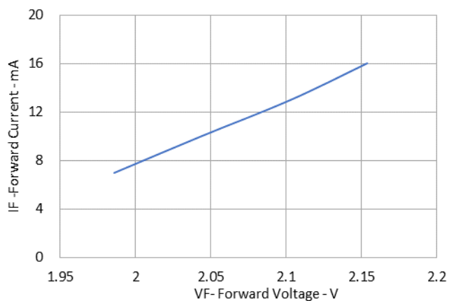
Fig.13 Input Current vs. Forward Voltage
