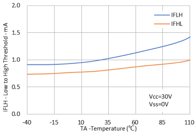
Fig.7 IFH vs. Temperature
