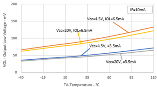
Fig.1 VOL vs. Temperature
