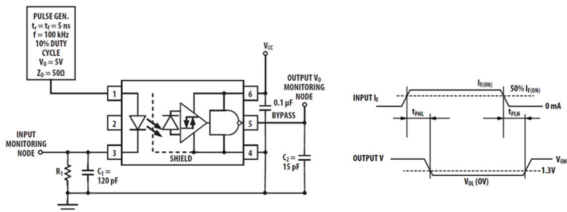
Fig.10 Test Circuit for t_{PHL} , t_{PLH} , t_r and t_f
