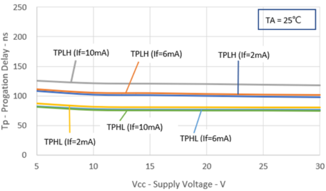
Fig.9 Propagation Delays vs. Vcc
