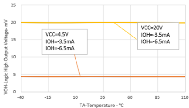
Fig.2 VOH vs. Temperature
