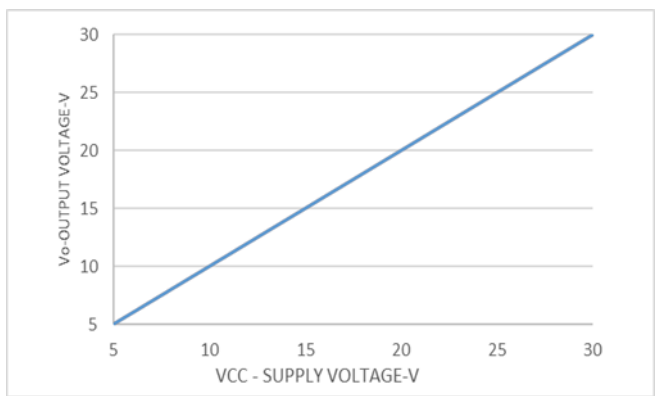
Fig. 6 Supply Voltage vs. Output Voltage
