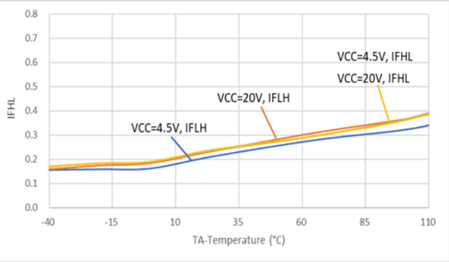
Fig.4 IFLH vs. Temperature
