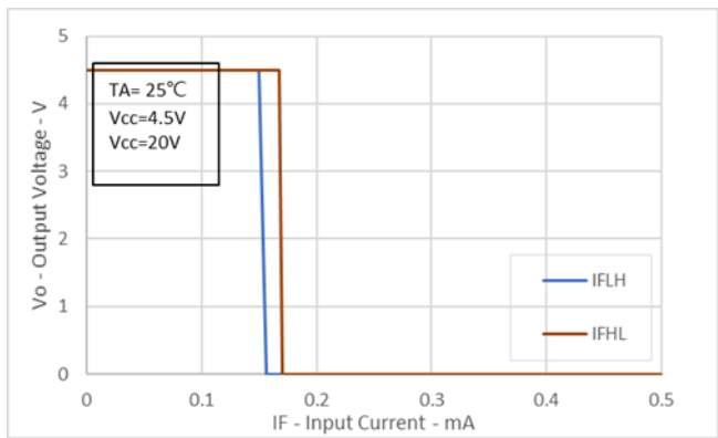
Fig.3 IFLH Hysteresis
