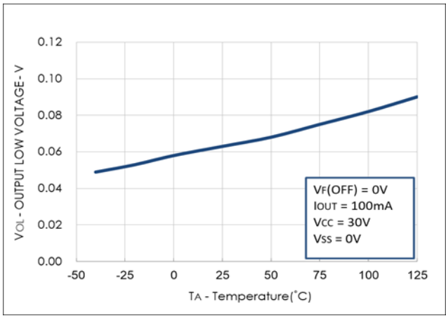
Fig.3 V OL vs. Temperature
